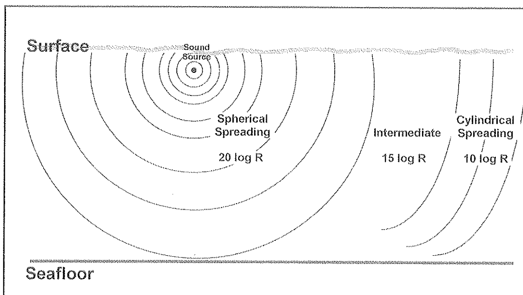
FIGURE 1. Schematic representation of acoustic spreading loss from a sound source as a function of distance and interaction with the seafloor (adapted from Davis et al. 1998). Note that distances are not drawn to scale.
