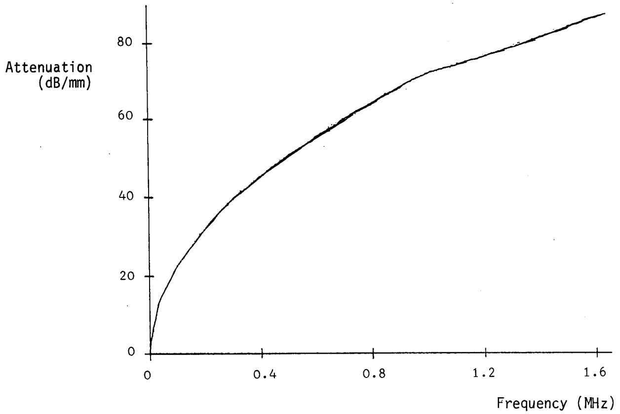
Fig. 5. Shear attenuation versus frequency for oil of viscosity 5 poise.
