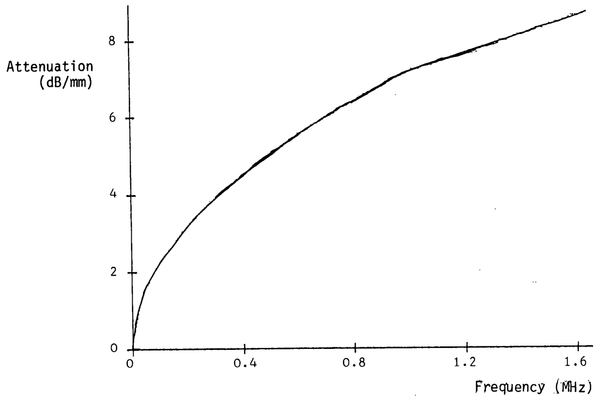
Fig. 6. Shear attenuation versus frequency for oil of viscosity 50 poise.
