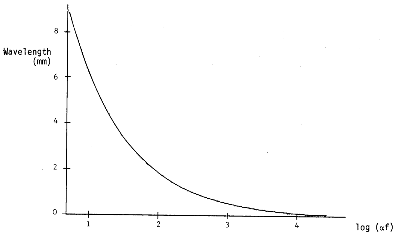
Fig. 12. Rayleigh wavelength in crude oil versus frequency.
