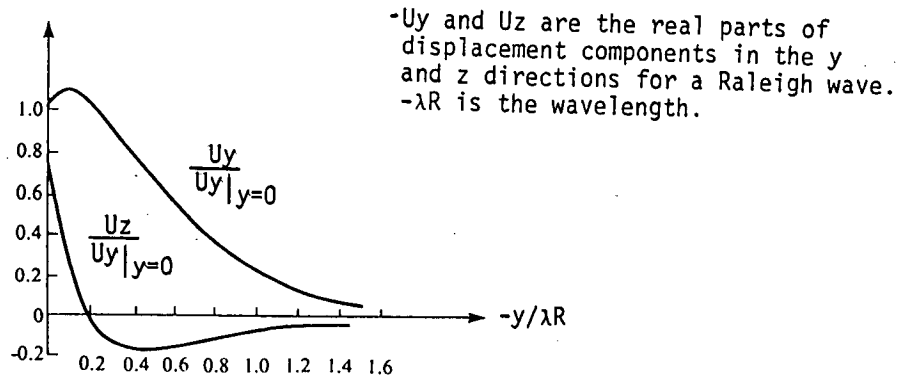
Fig. 11. Typical normalized displacements for a Rayleigh wave (from Ristic 1983).
