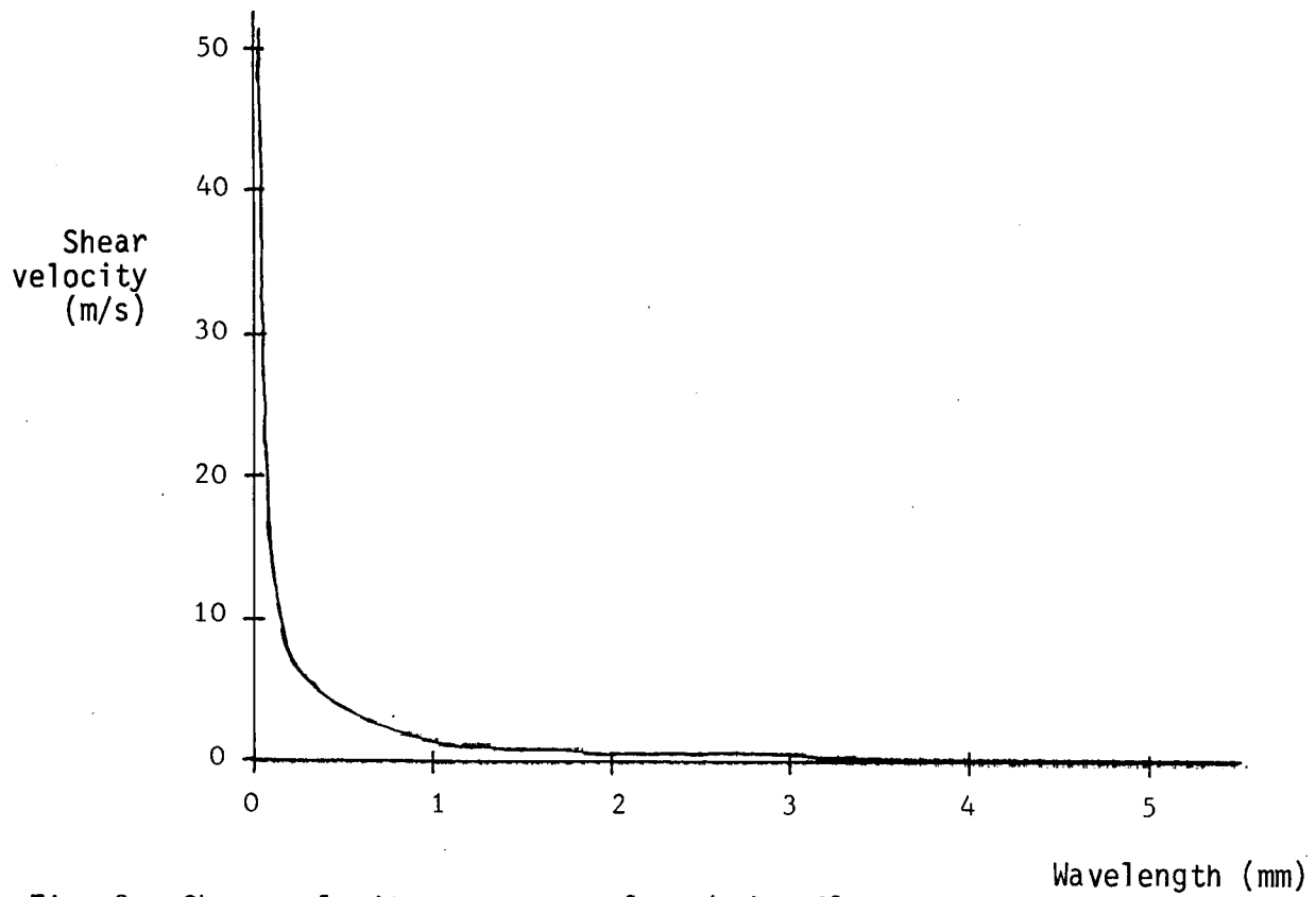
Fig. 3. Shear velocity versus wavelength in oil.
