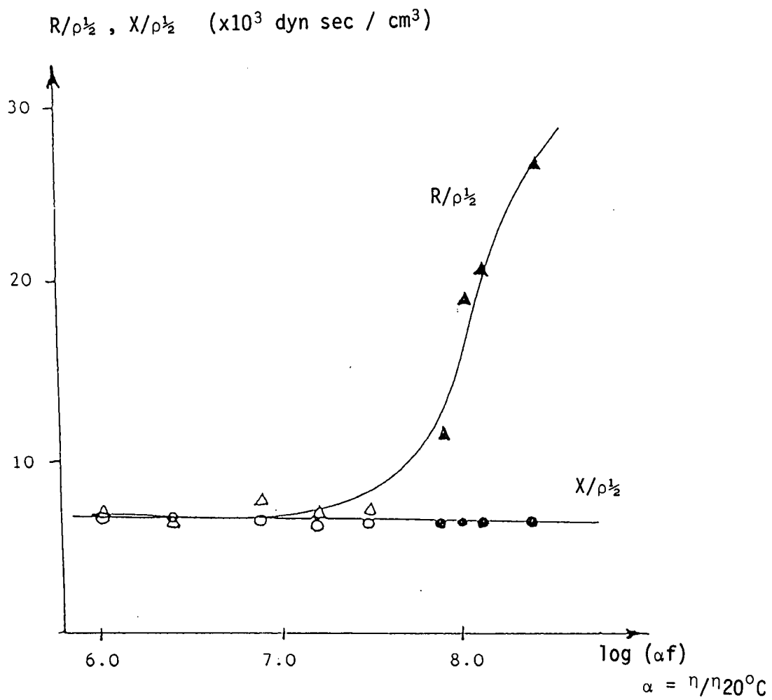
Fig. 2. Real and imaginary components of the shear mechanical impedance of crude oil, as a function of frequency (from Jones and Yeatman 1985).
