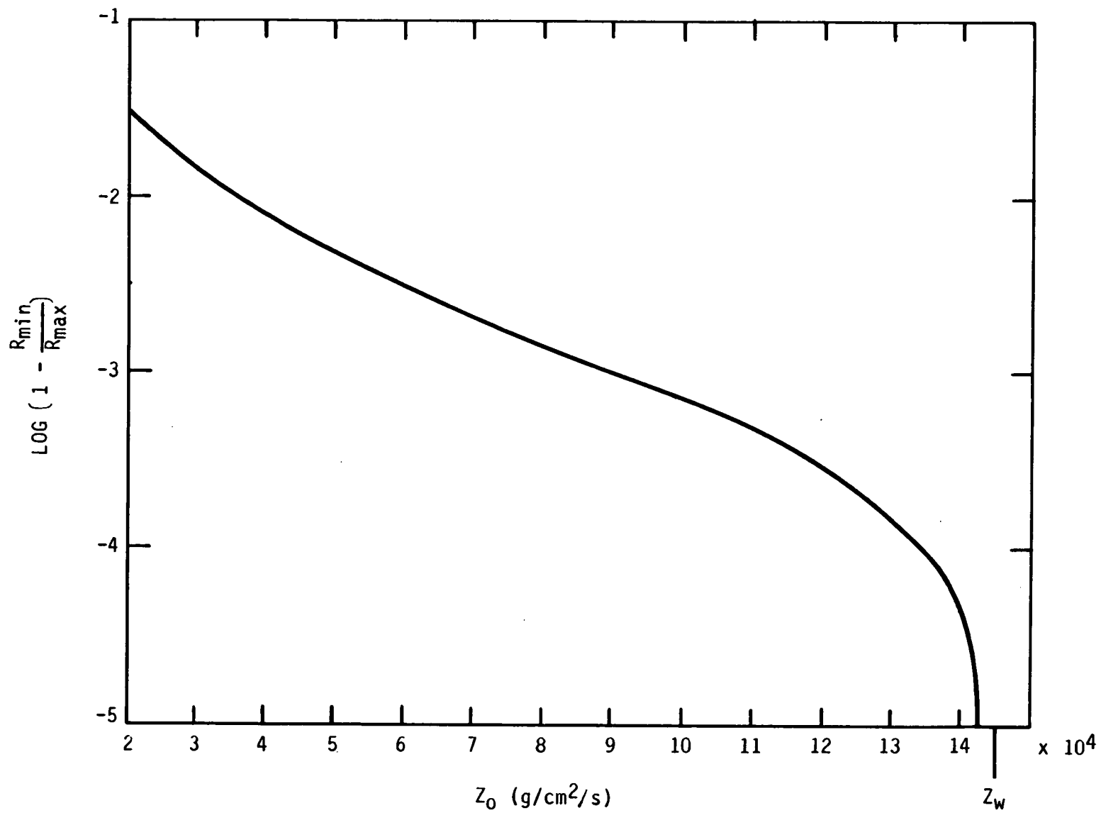
Fig. 27. Effect of changing the acoustic impedance of oil on the observable quantity (R_{\max} - R_{\min})/R_{\max} .
