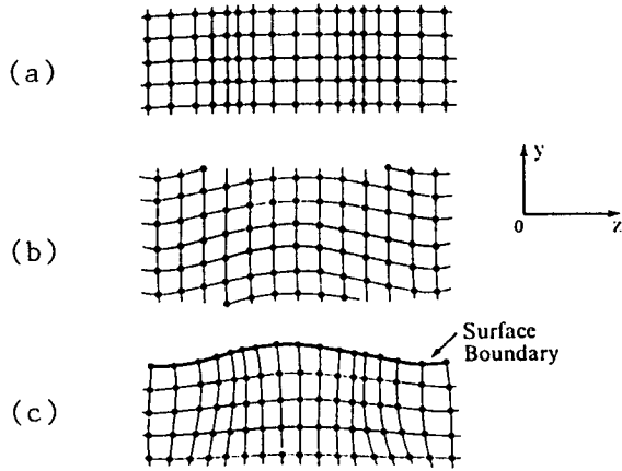
Fig. 10. Displacement patterns for (a) compressional wave, (b) y-polarized shear wave, and (c) Rayleigh wave, all propagating in the z direction (from Ristic 1983).
