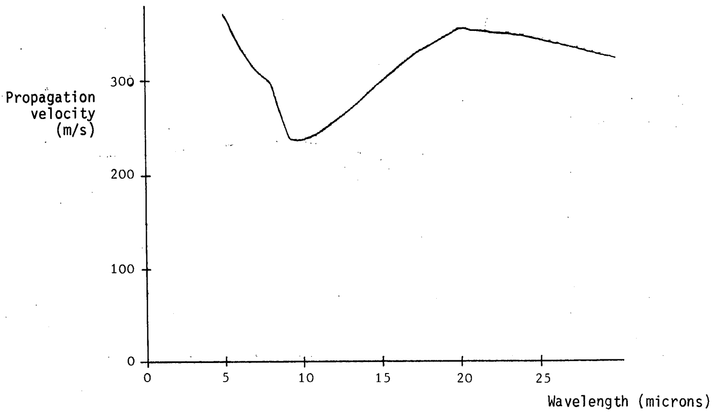
Fig. 16. Propagation of velocity of Lamb waves versus wavelength for an oil thickness of 10 microns.
