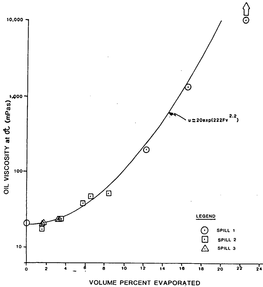
Fig. 9. Oil viscosity versus evaporation (from Buist and Bjerkelund 1986).
