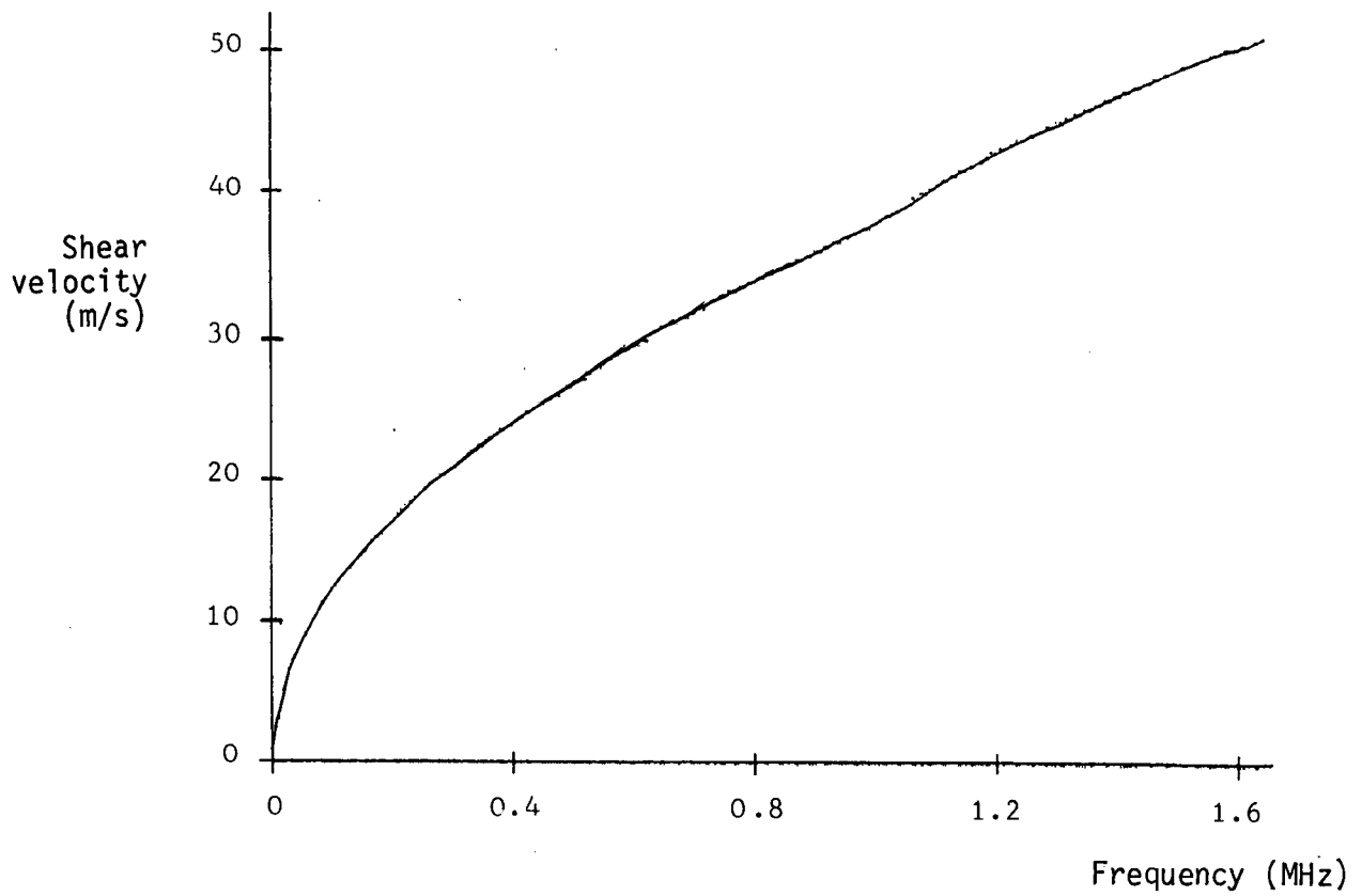
Fig. 4. Shear velocity versus frequency in oil.
