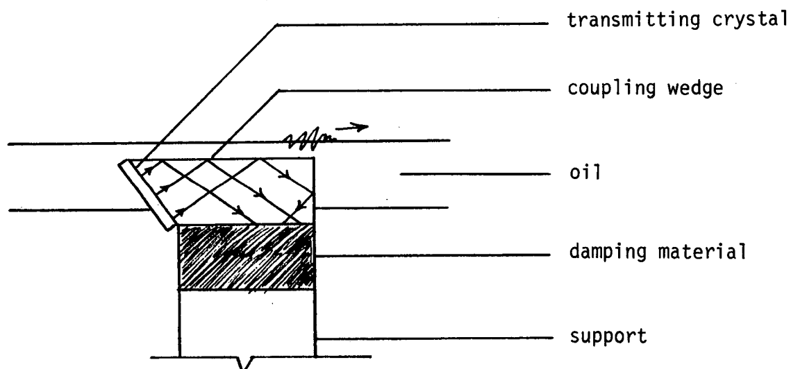
Fig. 22. The generation of SAWs using a compressional wave/wedge technique.
