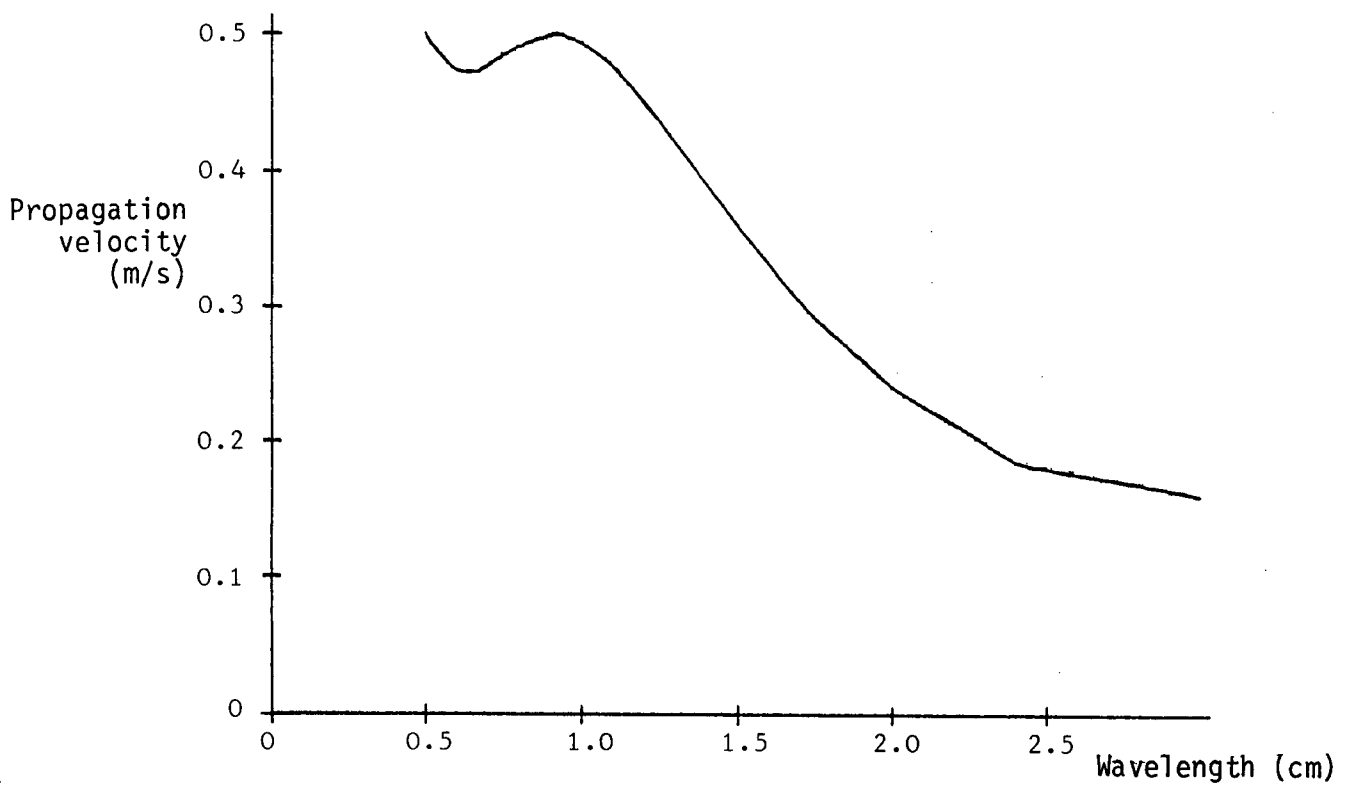
Fig. 19. Propagation velocity of Lamb waves versus wavelength for an oil thickness of 1 cm.
