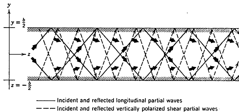
Fig. 15. Partial wave patterns for transverse resonance analysis of Lamb waves in a free layer (from Auld 1973).
