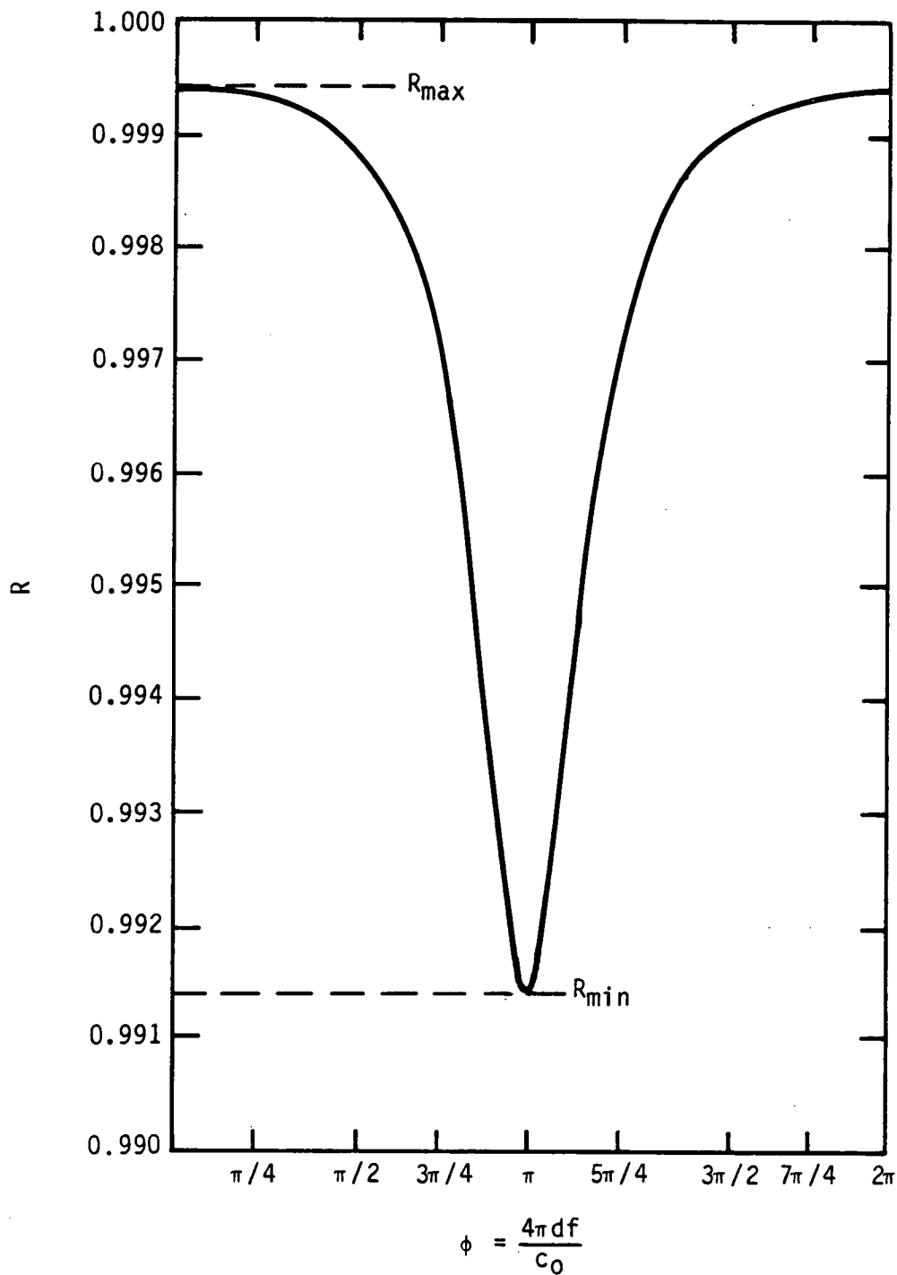
Fig. 26. Reflection coefficient plotted as a function of non-dimensionalized frequency: z_0 = 3.8 \times 10^4 \text{ g/cm}^2/\text{s} .
