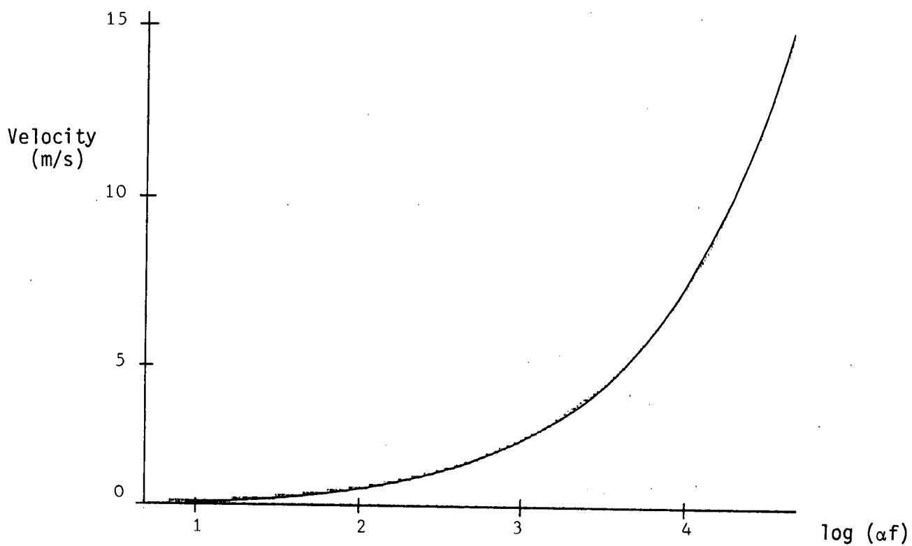
Fig. 13. Rayleigh wave velocity in crude oil versus frequency.
