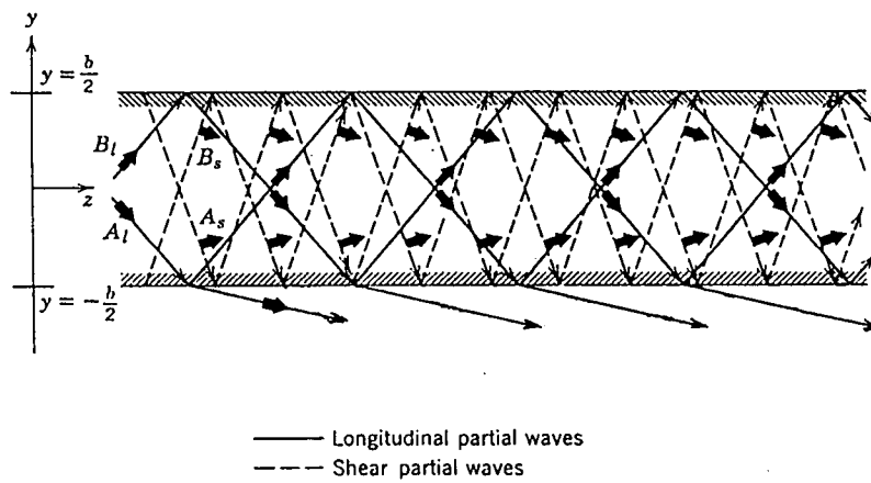
Fig. 20. Partial wave patterns for transverse resonance analysis of Lamb waves, in a layer bounded on one side by a water half-space (adapted from Auld 1973).
