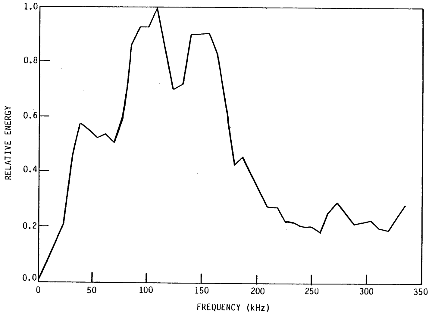
Fig. 28. Spectrum of acoustic energy generated by irradiating a water surface with a focused, pulsed CO 2 laser (Nebolsine et al. 1982).
