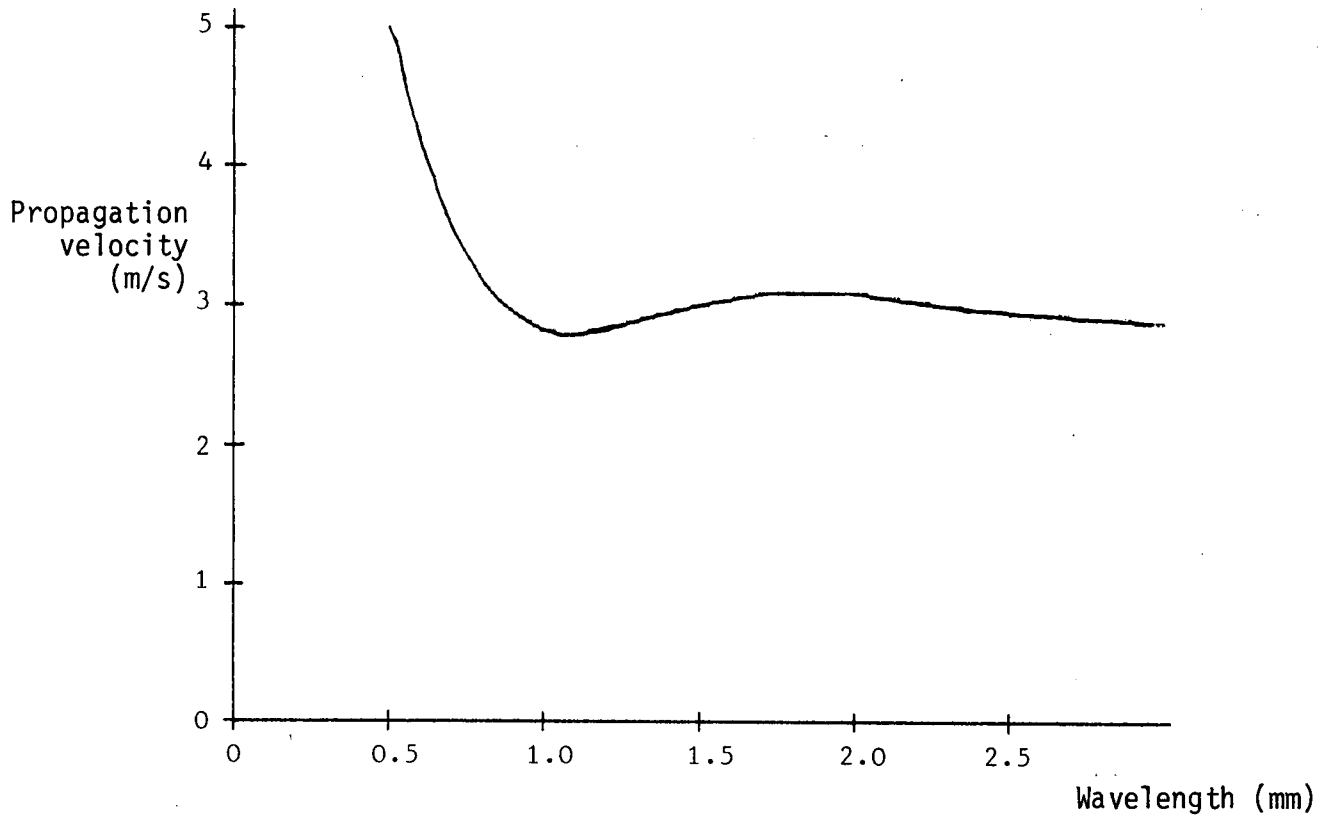
Fig. 18. Propagation velocity of Lamb waves versus wavelength for an oil thickness of 1 mm.
