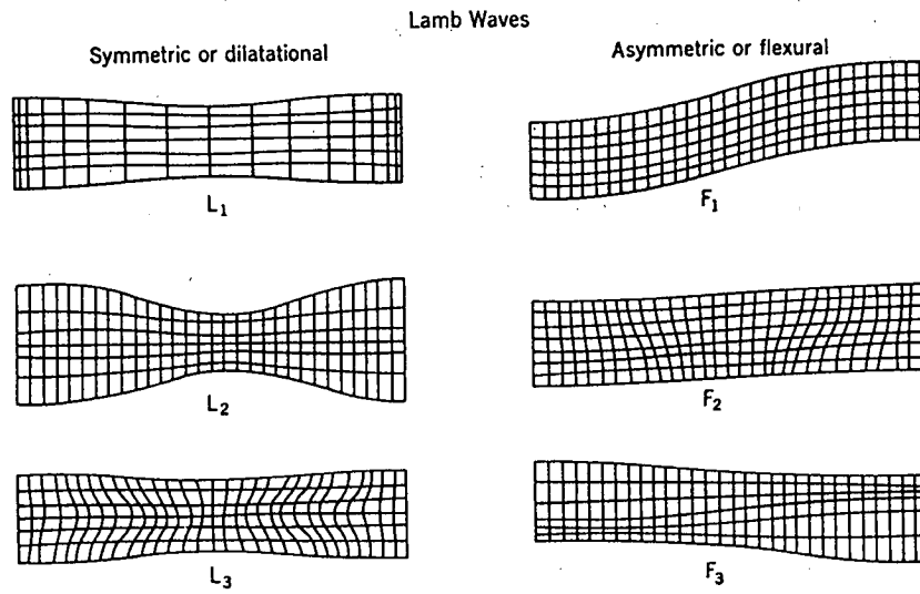
Fig. 14. Displacement patterns for the first three symmetric and asymmetric Lamb wave modes (from Auld 1973).
