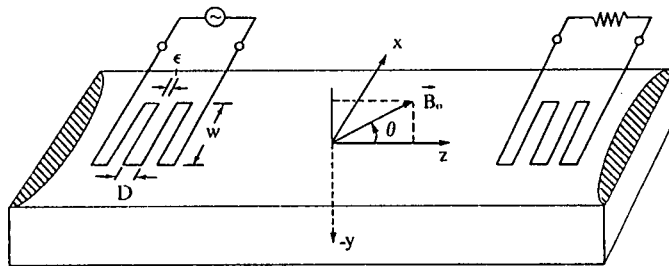
Fig. 21. Excitation of surface acoustic waves on a solid substrate (from Ristic 1983).
