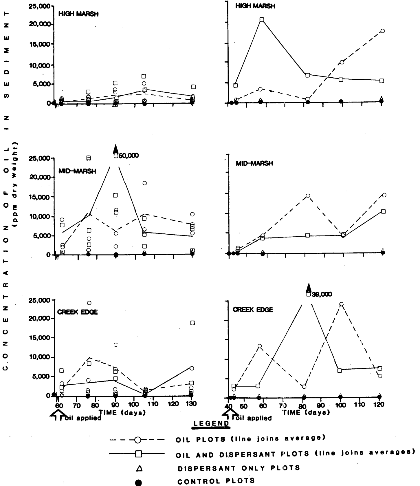
FIGURE 10 - OIL IN SEDIMENT RESULTS
