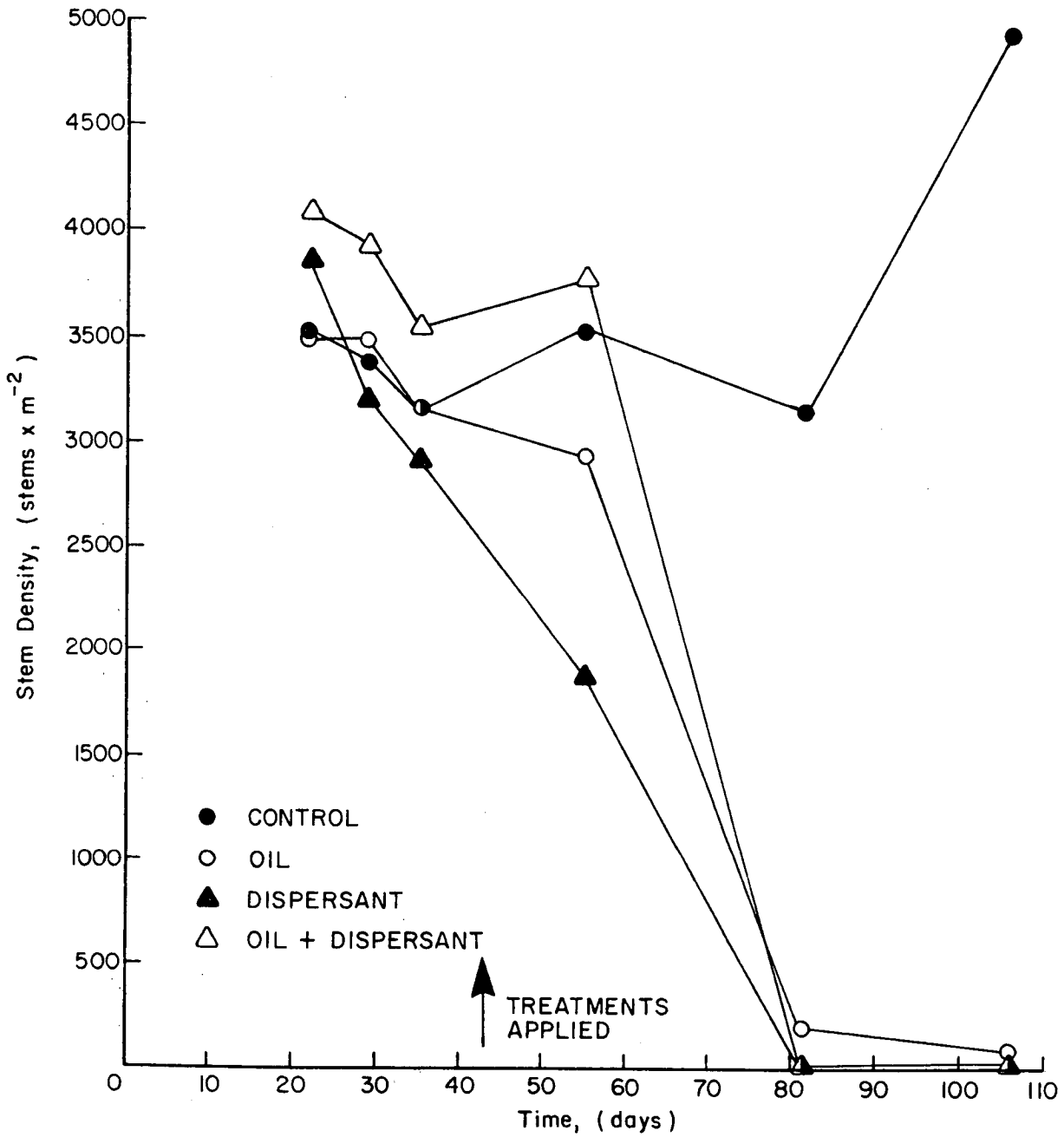
Figure 28: Mean stem density of Spartina alterniflora versus time. Data from control, oil and/or dispersant treated midmarsh zone greenhouse microcosms are presented. Treatments were applied on day 43.
